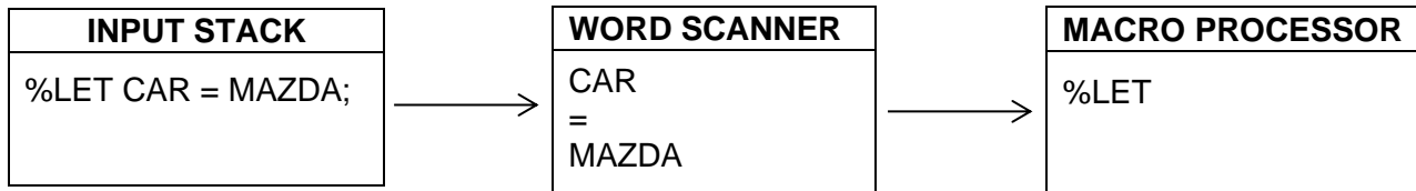
Figure 2. Macro tokens and the macro processor.
