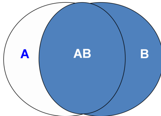
Figure 7. Venn Diagram – Right Outer Merge or Join
