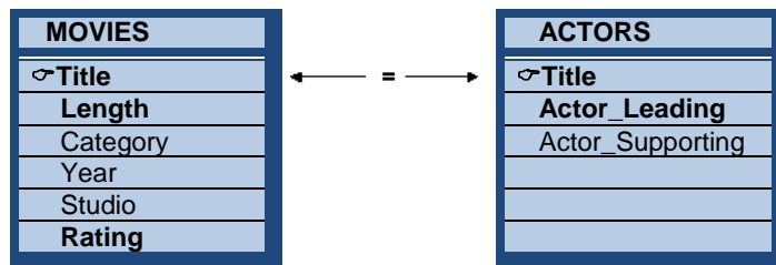
Figure 5. Matched Merge or Join using the MOVIES and ACTORS Tables
