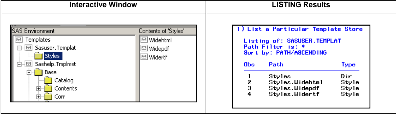
Figure 1: Comparison of Interactive Template Browser versus LIST Statement Output
